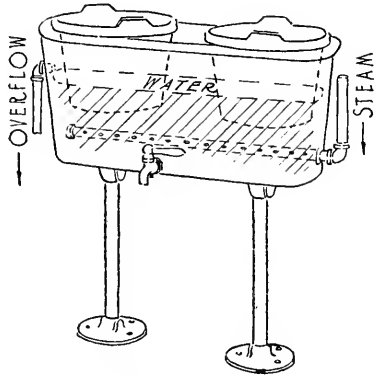
FIG. 130. STEAM GLUE HEATER.
